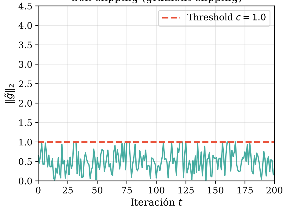
Con clipping (gradient clipping)
